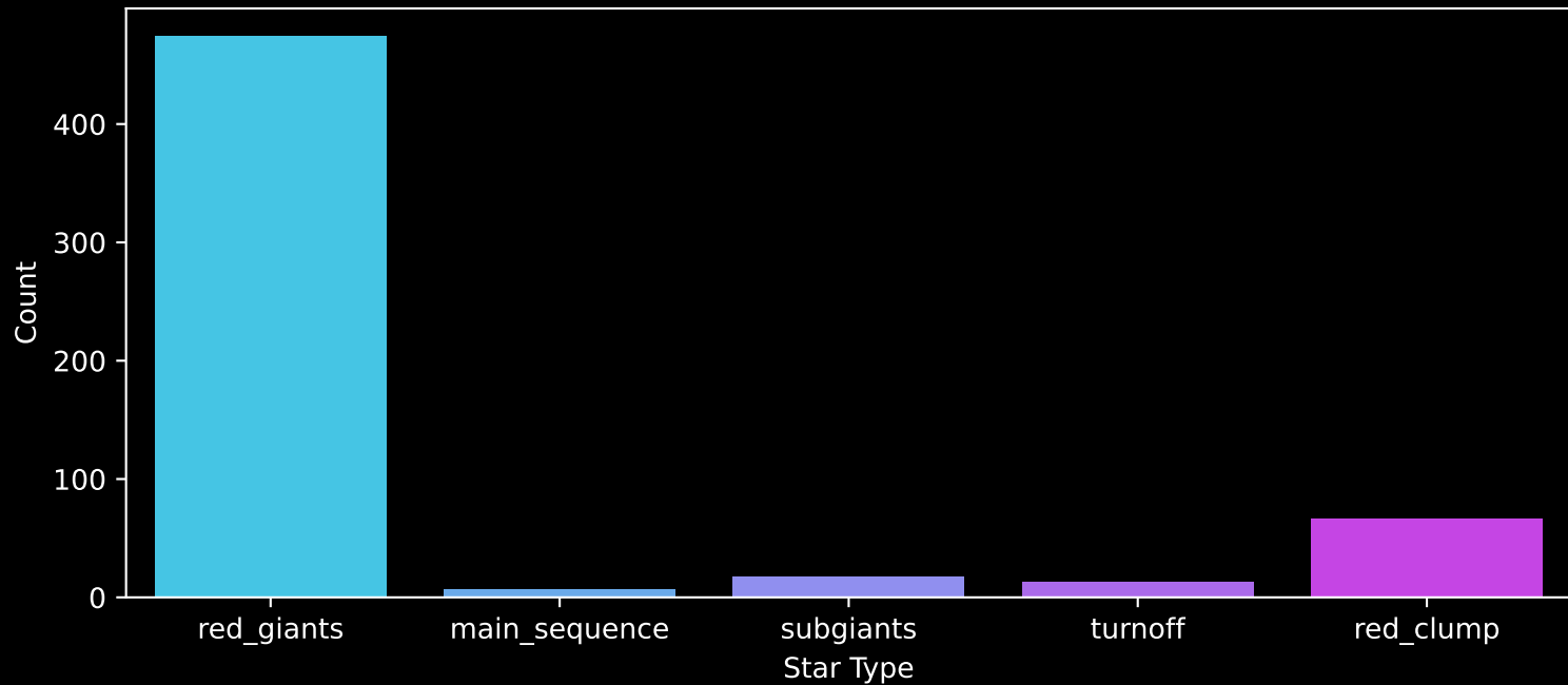
APOGEE DR17 Field: [330+04] Count plot of Star Type
