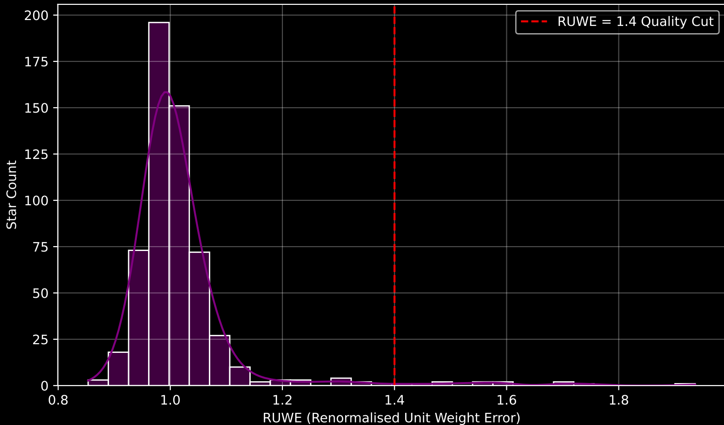
GAPOGEE DR17 Field [330+04] RUWE Distribution (n= 576)
