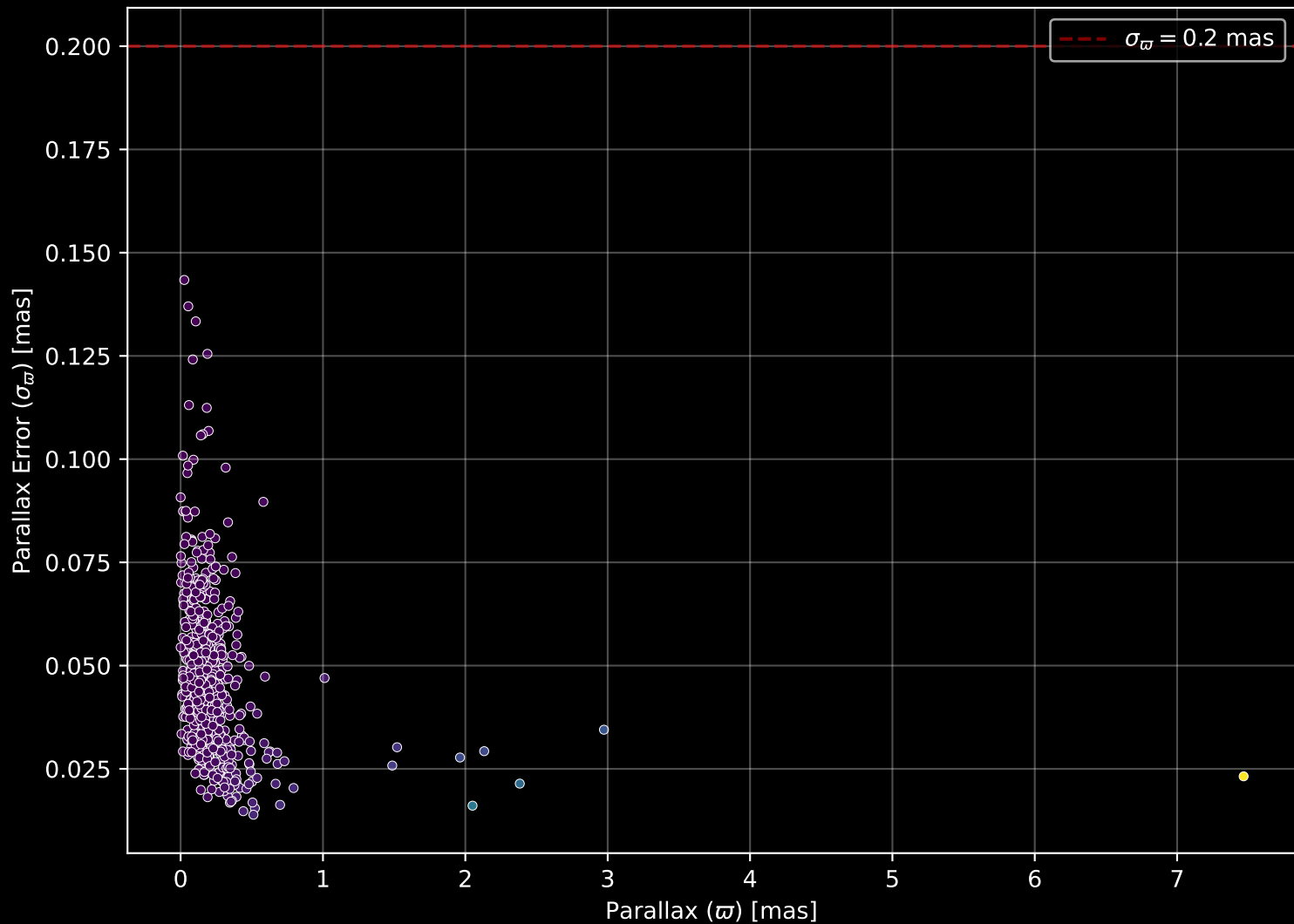
APOGEE DR17 Field: [330+04] Parallax Quality (n= 577)
