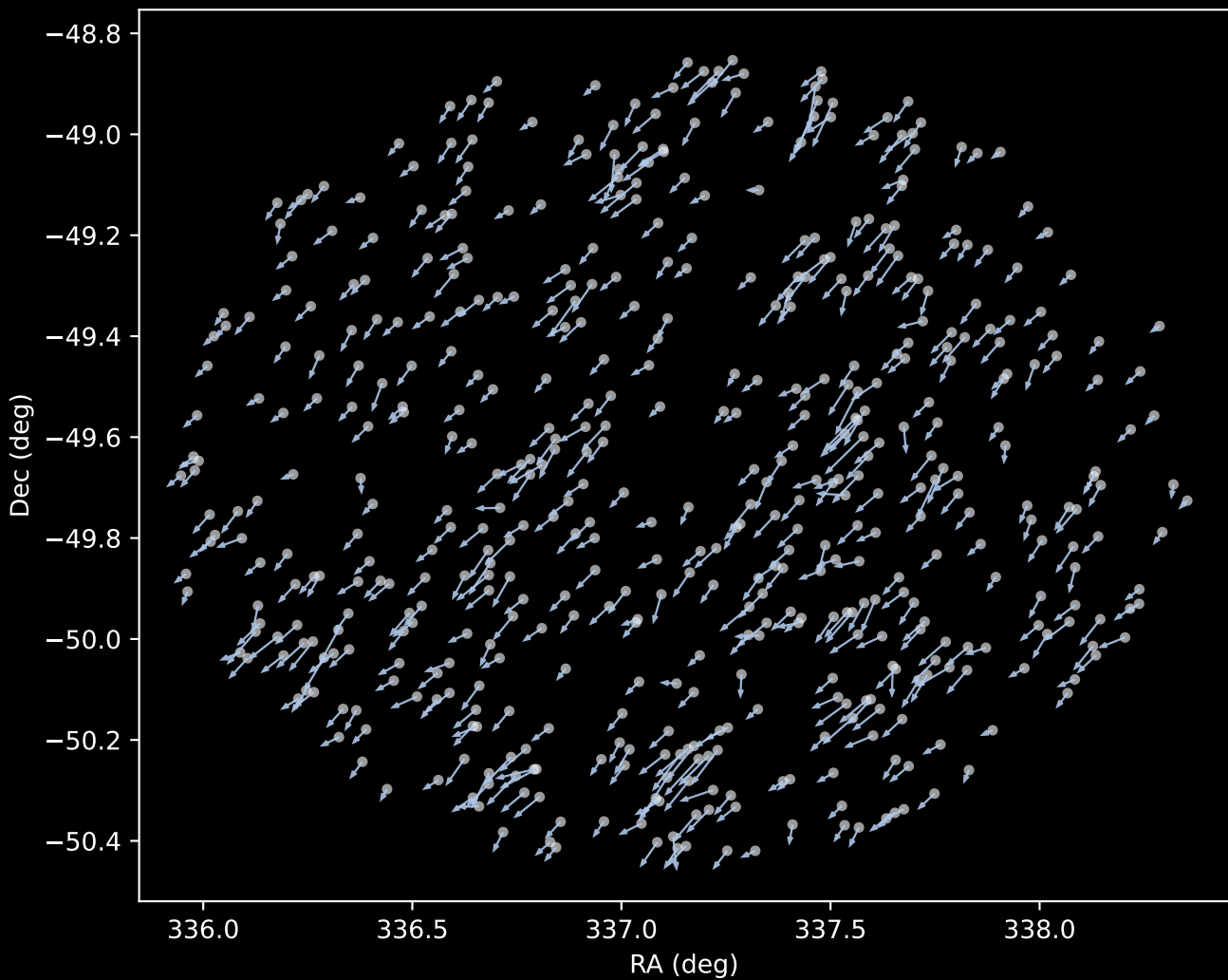
APOGEE DR17 Cluster 1 Proper Motion Vectors (n=512)
