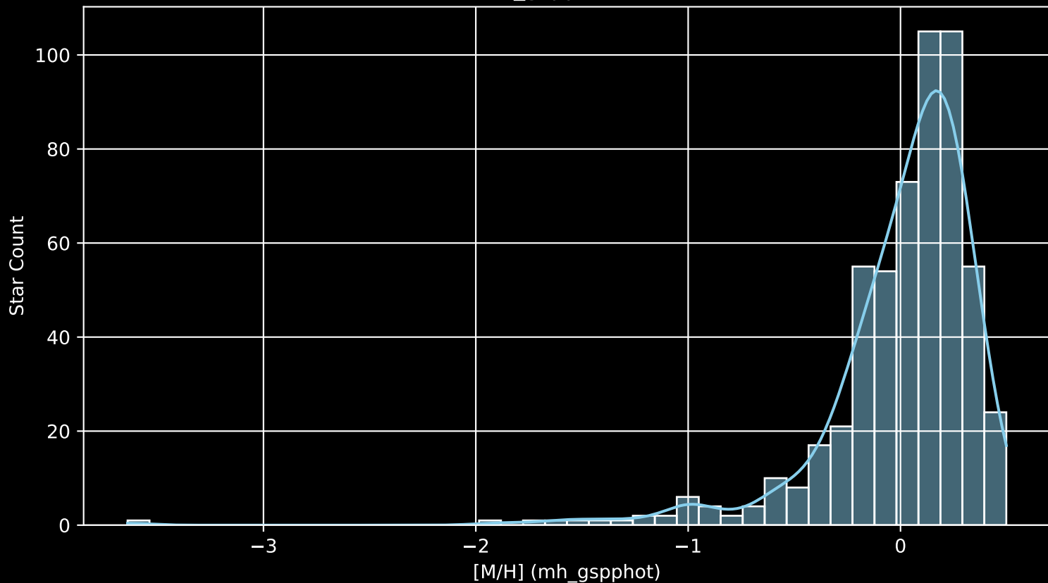
APOGEE DR17 Field: [330+04 [M/H] (mh_gspphot) (n= 554)
