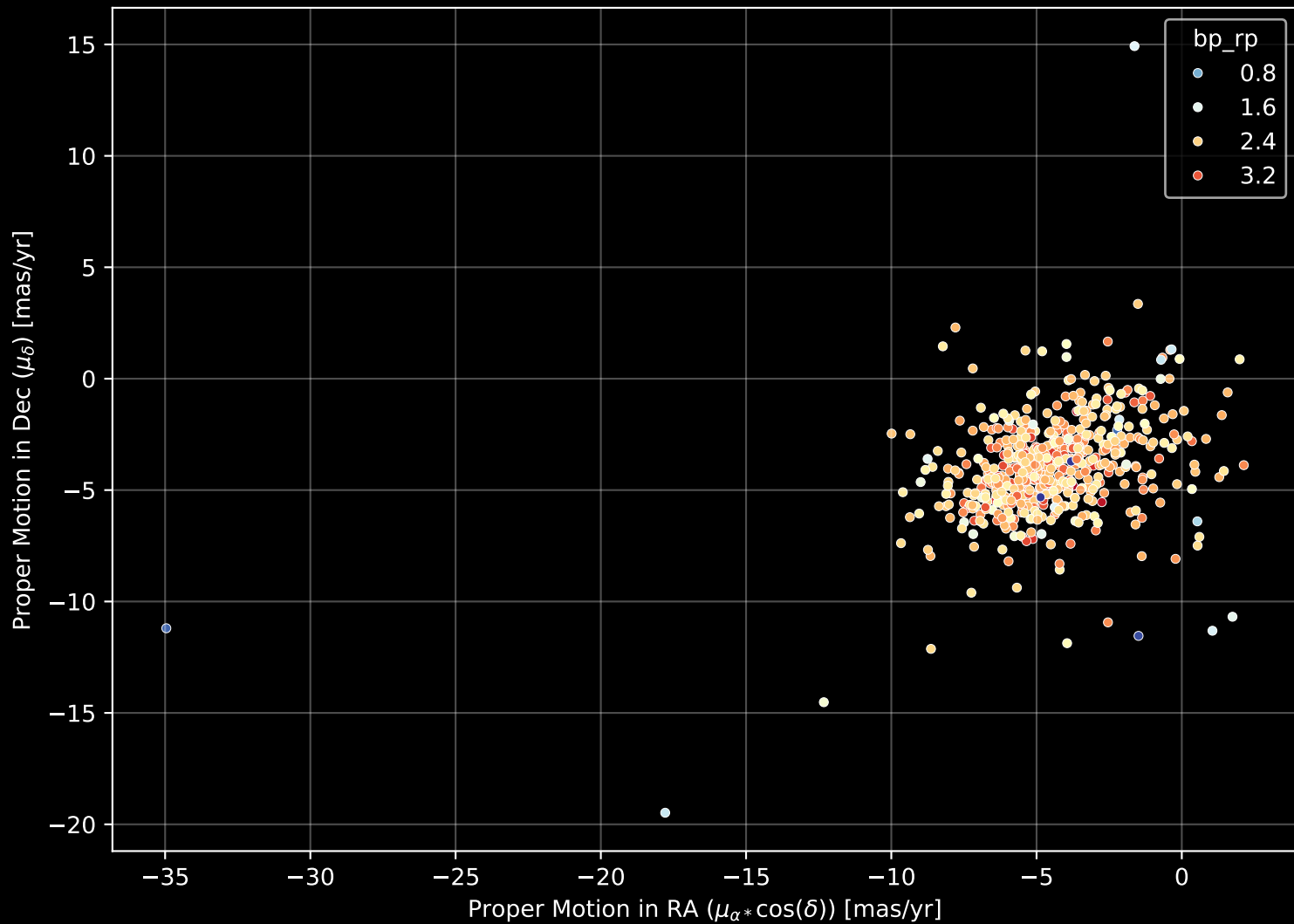
APOGEE DR17 Field: [330+04] Proper Motion Diagram (n= 577)
